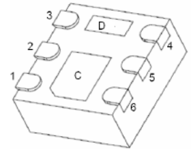
DFNWB2×2-6L-SA
